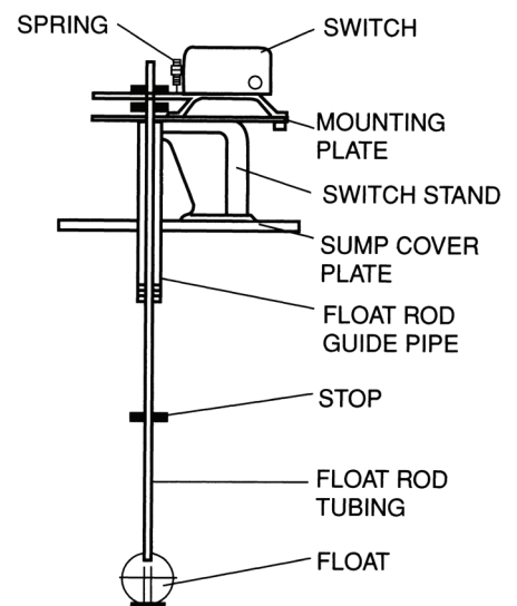
FLOAT SWITCH
